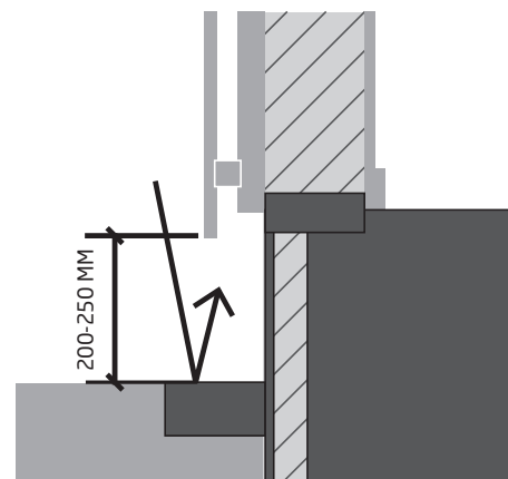
Recommended ground detail
