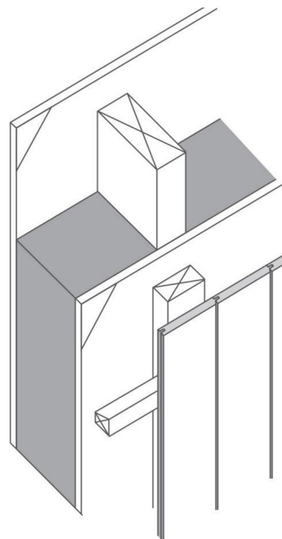
Recommended vertical boarding installation on double subframe.
