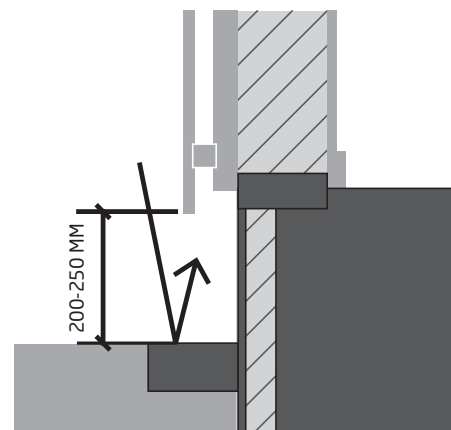
Recommended ground detail
