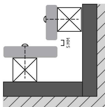
Typical external corner details
