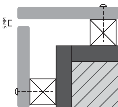
Typical external corner details
